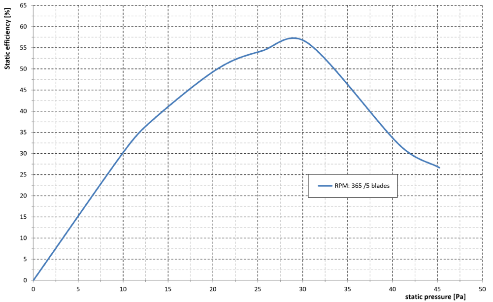
ERP Efficiency, static, A, %
