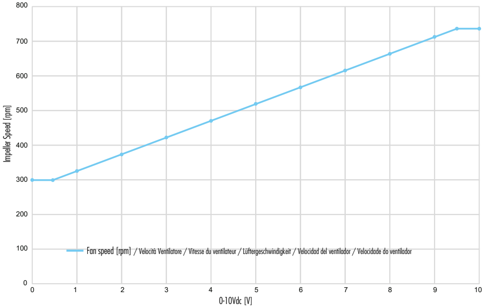
7 Speed Vs Voltage
