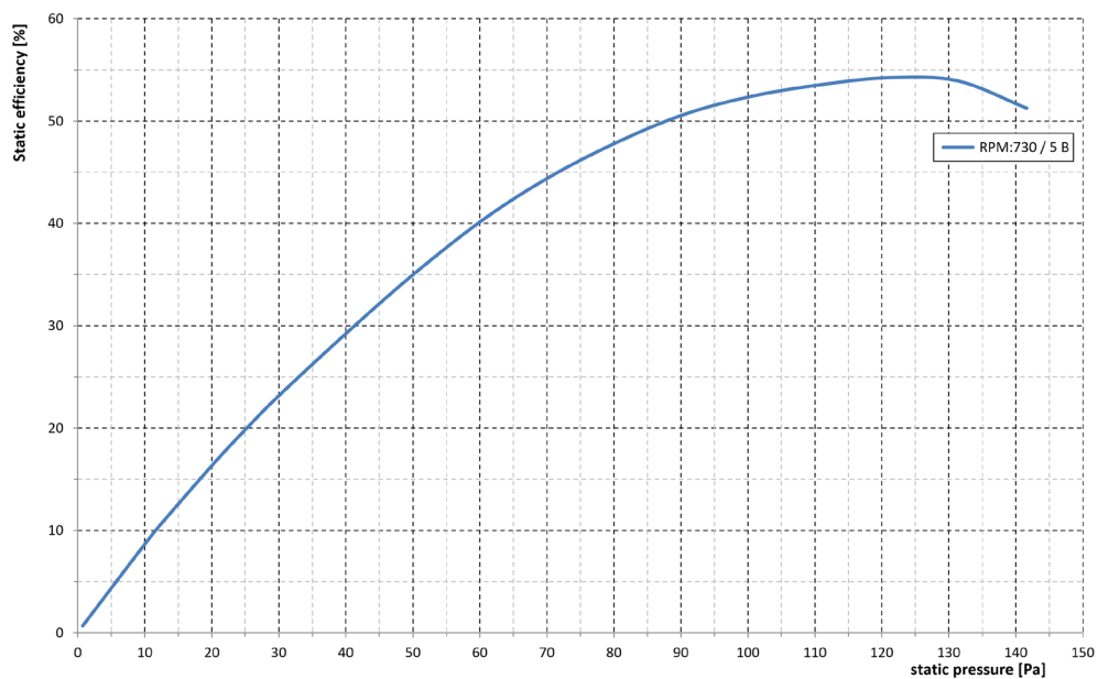
ERP Efficiency, static, %
